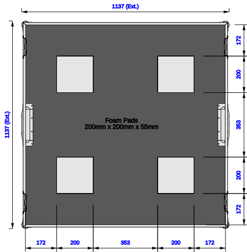
Door Foams centred so door can go on either way up
