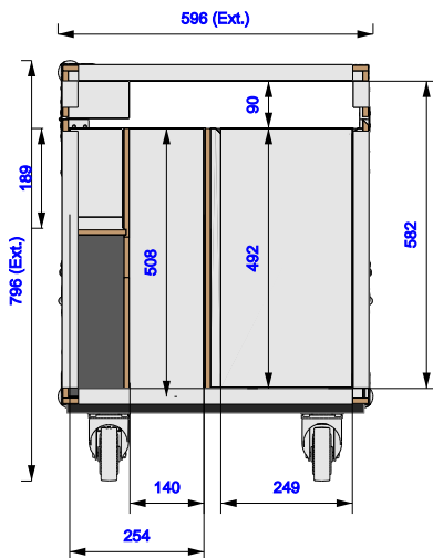
Cross section
