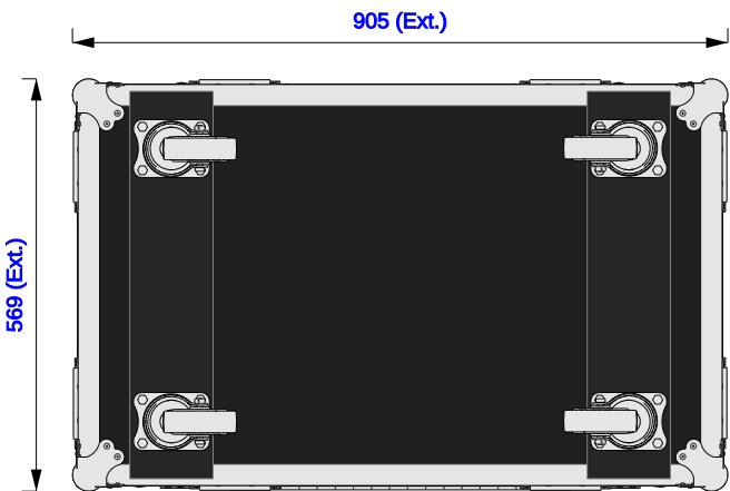
Underside
