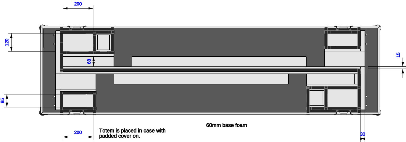
Right - Base only
