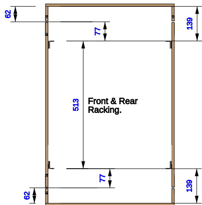
Rack Pitch.
