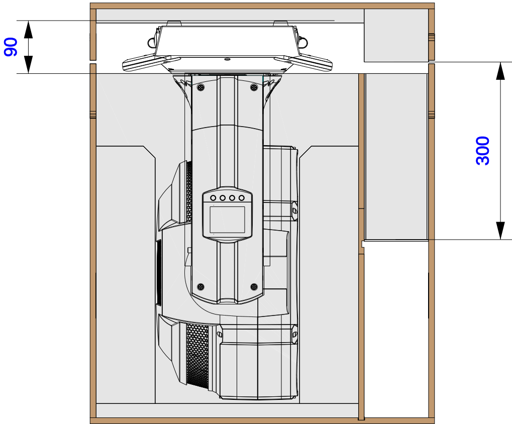
Right View with Kit Drawing.
