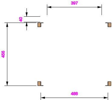
Rackstrip stating positions, plan view
