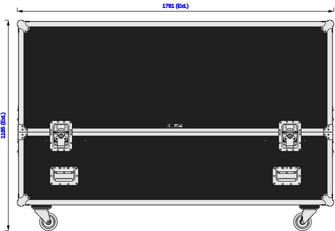
Front
