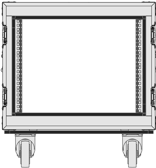
40D enclosure dimensions in mm [inch]
