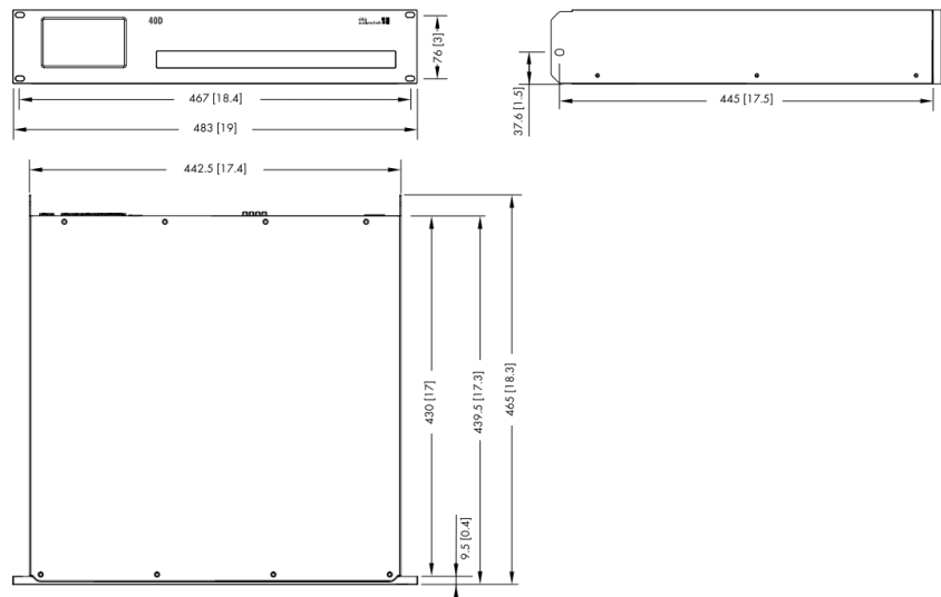
40D enclosure dimensions in mm [inch]
