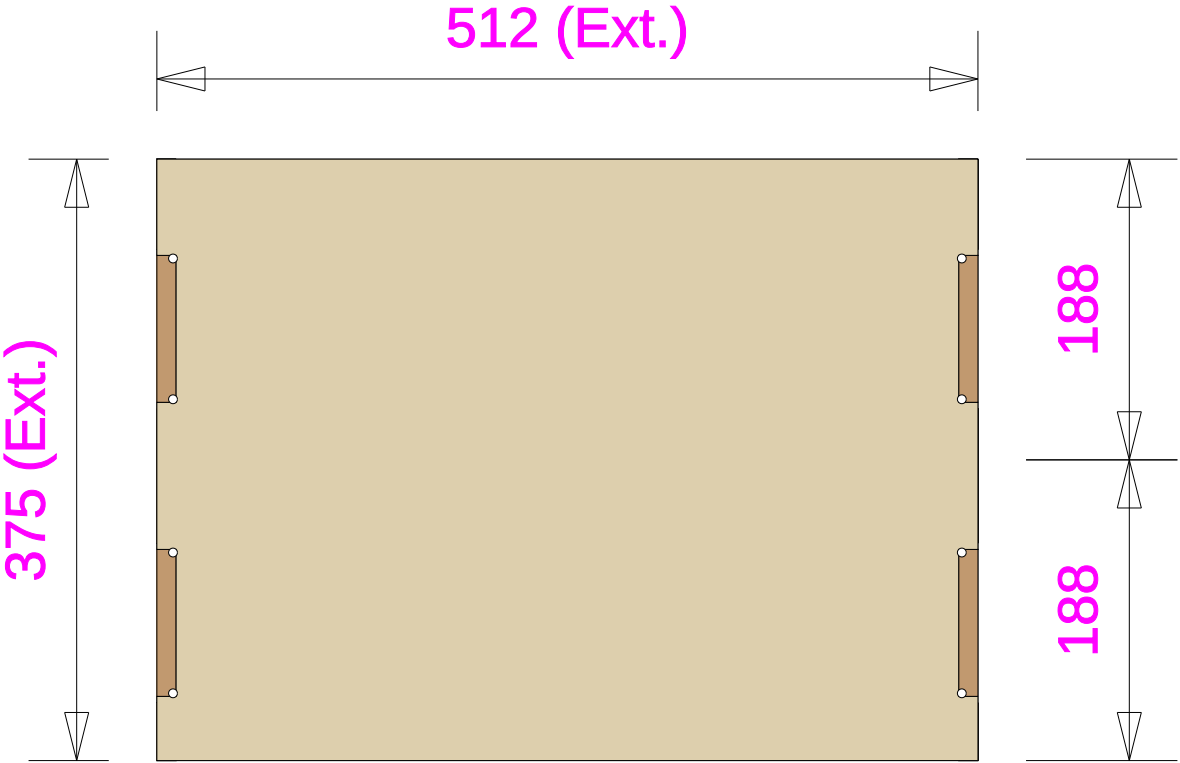
Underside
