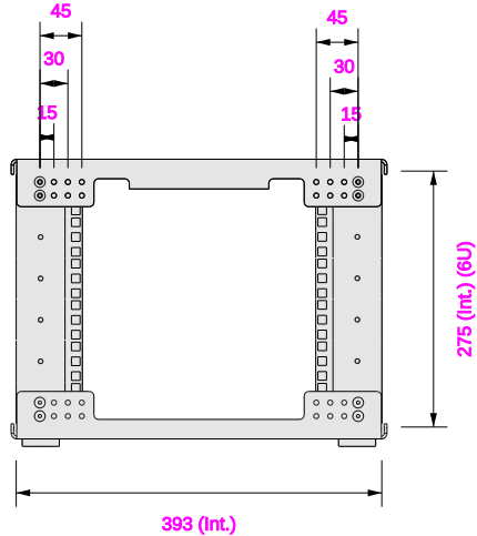
Adjustable depth front & rear Rack Rails
