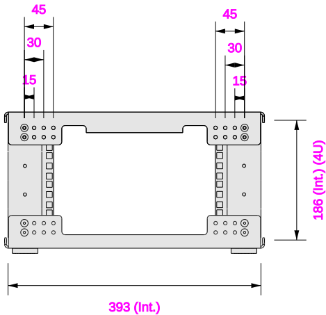
Adjustable depth front & rear Rack Rails
