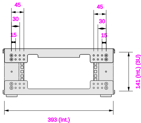
Adjustable depth front & rear Rack Rails
