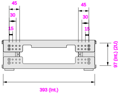
Adjustable depth front & rear Rack Rails
